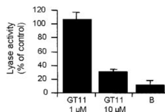
Fig. 7. Effect of GT11 on S1P lyase activity in primary cultured neurons. Cells were incubated in the absence (C, control) or presence of the indicated concentrations of GT11. After 24 h, cells were harvested, homogenized, and S1P lyase activity determined as described under Materials and Methods . B, blank with boiled homogenate. Data are from two separate experiments, each with double determinations.
