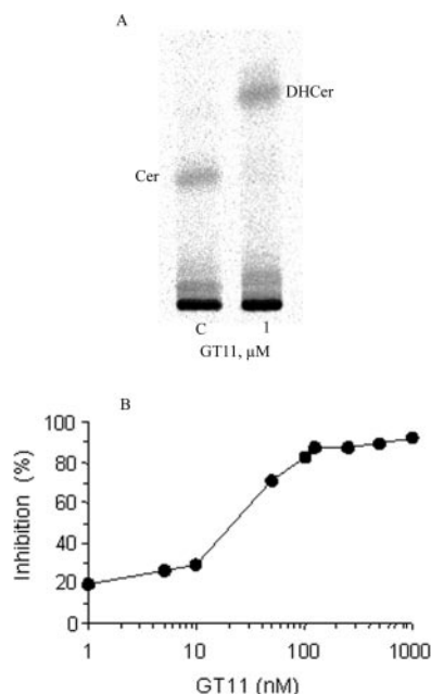
Fig. 2. Effect of GT11 on dihydroceramide desaturation in primary cultured neurons. Cells were incubated in the absence (C, control) or presence of the indicated concentrations of GT11. After 24 h, respective media were renewed and [ ^{14}\text{C} ]serine added for additional 24 h. Then, cells were harvested and lipids extracted and isolated as described in Materials and Methods . Ceramide (Cer) was separated from dihydroceramide (DHCer) by TLC on borate-treated silica gel plates with chloroform/methanol (9:1, by volume) as solvent system. The radioactively labeled ceramide and dihydroceramide were quantitatively evaluated as described in Materials and Methods . Inhibition of desaturation of DHCer to Cer was calculated relative to controls. The results are given as the mean of double determinations from one representative experiment that was repeated twice with similar results. The standard deviation values were always in the range of \pm 5\% of the mean.
