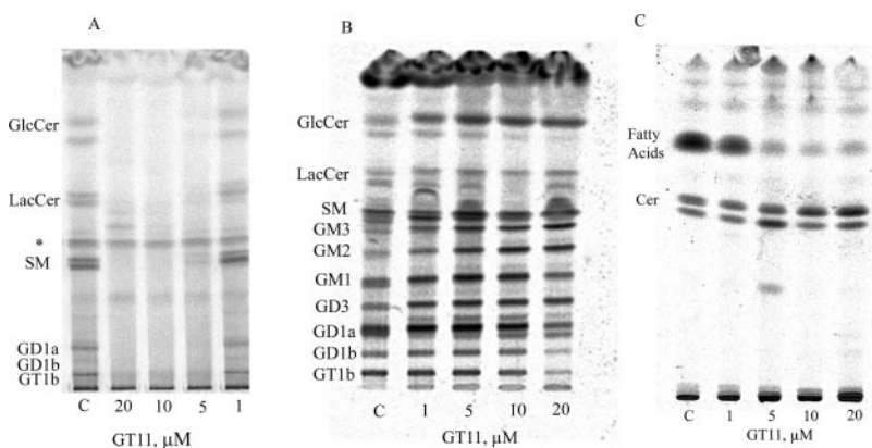
Fig. 3. Effect of GT11 on [ ^{14}\text{C} ]serine and [ ^3\text{H} ]sphinganine incorporation into cellular sphingolipids. Primary cultured neurons were incubated in the absence (C, control) or presence of the indicated concentrations of GT11. After 24 h, 1 \mu\text{Ci} of either [ ^{14}\text{C} ]serine (A) or [ ^3\text{H} ]sphinganine (B and C) was added to the renewed medium. Twenty-four hours later, cells were harvested and lipids were extracted, isolated, separated by TLC, and detected as described under Materials and Methods . The solvent system used was chloroform/methanol/0.22% aqueous \text{CaCl}_2 , 60:35:8, by volume (A and B) or chloroform/methanol/acetic acid, 190:9:1, by volume (C). The terminology of gangliosides (GT1b, GD1b, GD1a, GD3, GM1, GM2, and GM3) is according to Svennerholm (1963). Other abbreviations are as follows: SM, sphingomyelin; LacCer, lactosylceramide; GlcCer, glucosylceramide; *, unidentified bands.
