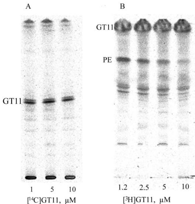
Fig. 5. Metabolism of radioactively labeled GT11 in primary cultured neurons. Cells were incubated in the presence of the indicated concentrations of GT11, including 5 nCi of [ ^{14}\text{C} ]GT11 (A) or 0.72 \mu\text{Ci} of [ ^3\text{H} ]GT11 (B), respectively. After 24 h, cells were harvested and lipids were extracted, isolated, separated by TLC (A: chloroform/methanol/acetic acid, 190:9:1, by volume; B: chloroform/methanol/0.22% aqueous \text{CaCl}_2 , 60:35:8, by volume), and detected as described under Materials and Methods . Note that alkaline treatment was omitted to keep phospholipids intact.
