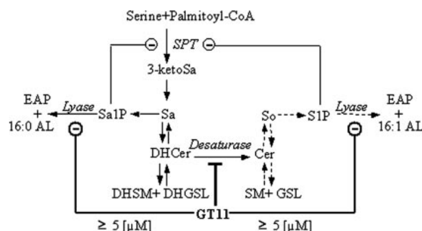
Fig. 9. Proposed mechanism for the effect of GT11 on sphingolipid metabolism in primary cultured cerebellar neurons. At submicromolar concentrations (1–1000 nM), GT11 specifically inhibits dihydroceramide desaturase. At concentrations above 5 \mu M, GT11 also decreases lyase activity. This effect results in the accumulation of sphingoid-1-phosphates, which down-regulate SPT. Note that an accumulation of S1P is possible despite a complete inhibition of dihydroceramide desaturase from catabolic ceramide pools formed by breakdown of sphingomyelin (SM) and of glycosphingolipids (GSL). AL, aldehyde; EAP, ethanolamine phosphate; (DH)Cer, (dihydro)ceramide; (DH)GSL, (dihydro)glycosphingolipids; (DH)SM, (dihydro)sphingomyelin; Sa, sphinganine; Sa1P, sphinganine-1-phosphate; So, sphingosine; S1P, sphingosine-1-phosphate.
