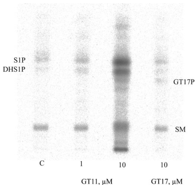
Fig. 6. Determination of ^{32}\text{P}_i -labeled sphingoid phosphates in primary cultured cerebellar neurons. Cells were washed with phosphate-free MEM and incubated with the same medium containing ^{32}\text{P}_i (40 \mu\text{Ci}/\text{ml} ) for 24 h. Then, vehicle (lane C) or the indicated concentration of GT11 or GT17 was added for 24 h. Cells were harvested and sphingosine phosphates extracted, resolved by TLC, and determined as described under Materials and Methods . The R_f value of authentic sphingoid phosphates is indicated. Similar data were obtained in two separate experiments, each with double determinations.
