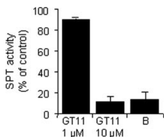
Fig. 4. Effect of GT11 on SPT activity in primary cultured neurons. Cells were incubated in the absence (C, control) or presence of the indicated concentrations of GT11. After 24 h, cells were harvested, homogenized, and enzyme activity determined as described under Materials and Methods . B, blank with boiled homogenate. Data are from three separate experiments, each with double determinations.
