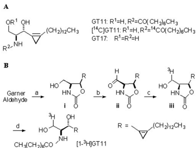
Fig. 1. Chemical structure (A) and synthesis of [ ^3\text{H} ]GT11 (B). The tritiated GT11 analog was prepared from the cyclic carbamate (i). Oxidation (b, Dess-Martin periodinane, \text{CH}_2\text{Cl}_2 ) to the aldehyde (ii) and its further reduction (c, \text{NaB}^3\text{H}_4/\text{methanol} ) yielded the tritiated alcohol (iii), which, upon deprotection and acylation, afforded [ ^3\text{H} ]GT11. Reagents and conditions of the reactions a and d are as described by Triola et al. (2001, 2003).
