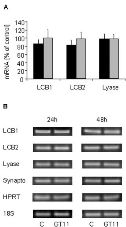
Fig. 8. Effect of GT11 on mRNA levels of SPT and S1P lyase in primary cultured neurons. Cells were incubated for the indicated times (black columns, 24 h; gray columns, 48 h) in the absence (control) or presence of 10 \mu M GT11. After 24 h, respective media were renewed. Levels of SPT (LCB1 and LCB2) and of S1P lyase mRNA were determined by quantitative real-time PCR (A) and by semiquantitative RT-PCR (B) as described under Materials and Methods . A, data are means from three different experiments, each with triple determinations. B, one representative of three experiments with similar results from different cell preparations. C, control; HPRT, hypoxanthinephosphoribosyltransferase; LCB, long-chain base; Synpto, synaptophysin; 18S, 18S rRNA.
